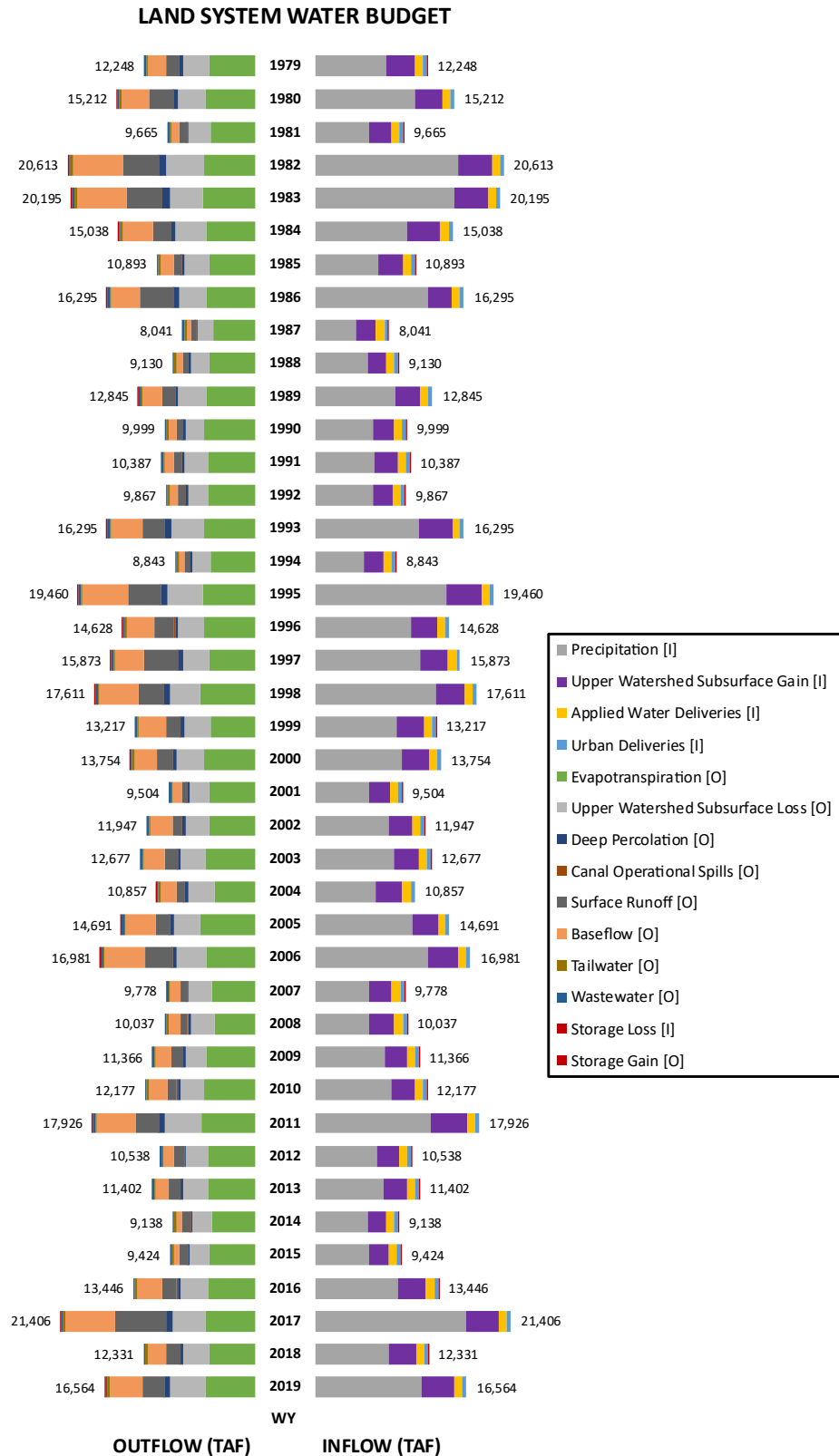
Figure 5-2. ABC WRP Total Historical Land System Water Budget between Water Years 1979 and 2019
