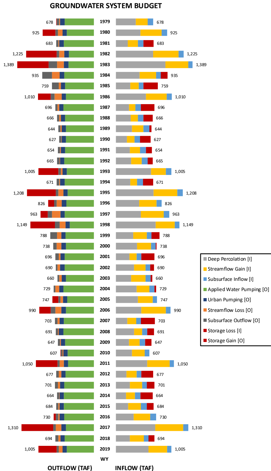
Figure 5-3. ABC WRP Total Historical Groundwater System Budget between Water Years 1979 and 2019
